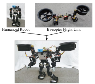
Transform robot
