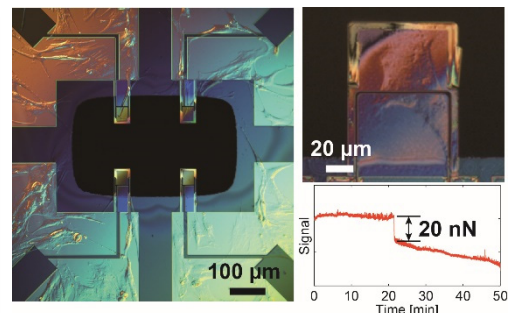
Real-time measurement of traction force generated by bovine aortic smooth muscle cells.
