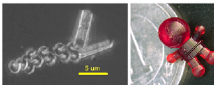
micro humanoid fabricated by micro stereolithography
