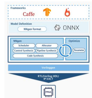
NNgen: DNN-HW Synthesis Compiler
